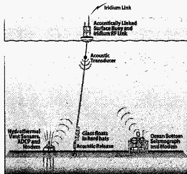
Fig. 1. Conceptual drawing of an acoustically-linked observatory.
