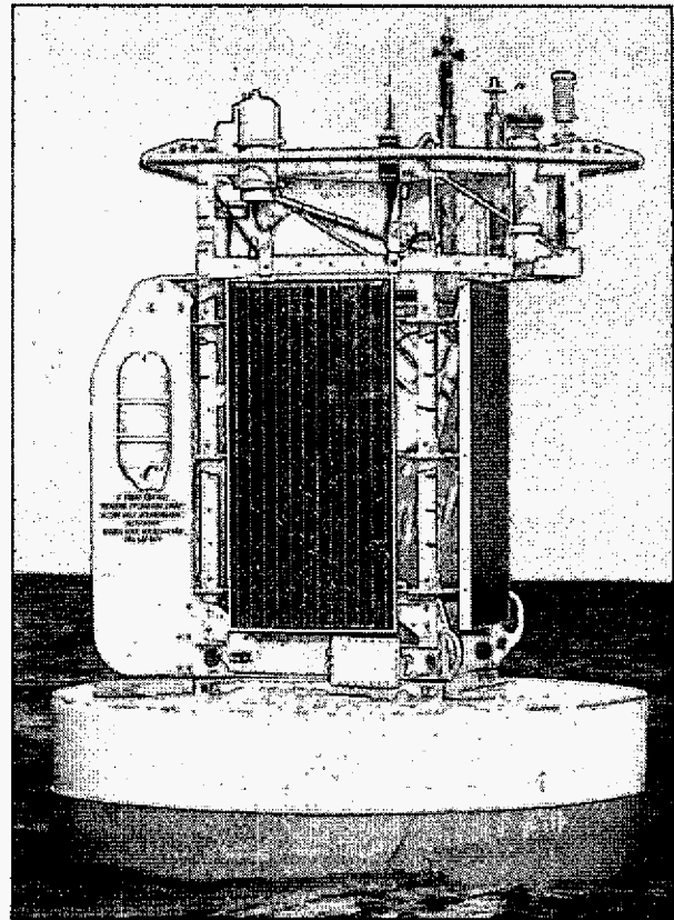
Fig. 3. Buoy with solar panels, meteorological sensors and antennas.
